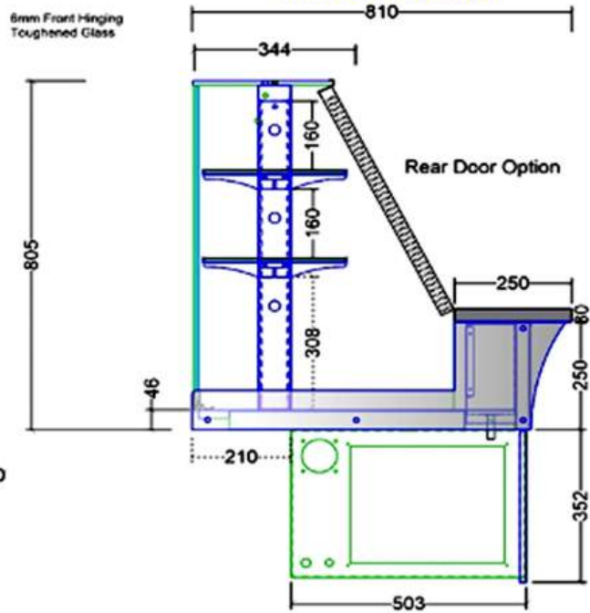
SIDE VIEW CC Drop-in-2S Refrigerated Base Two Ambient Shelves
