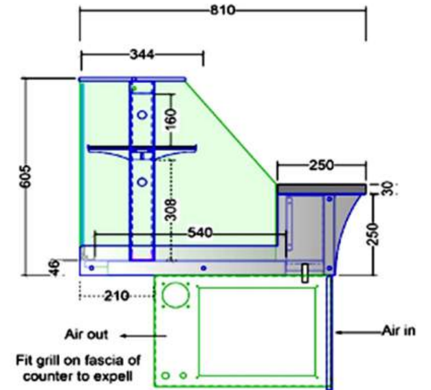
SIDE VIEW CC Drop-in-1S Refrigerated Base One Ambient Shelves
